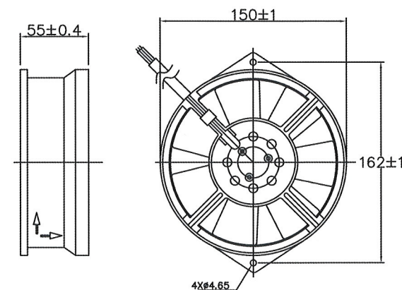
Dimensions (mm)
