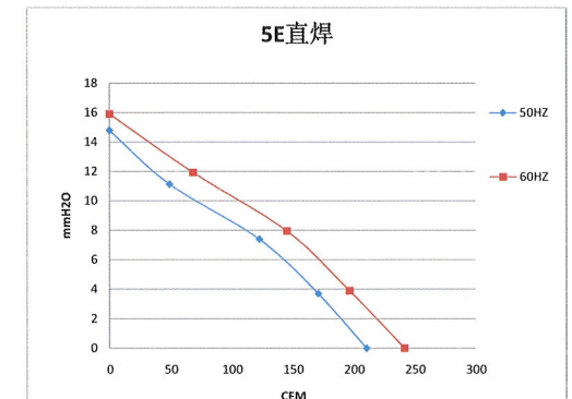
Performance Curve
