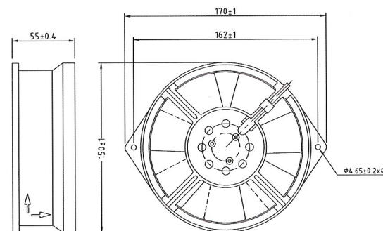
Dimensions (mm)
