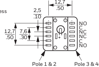
0.020 in x 0.110 in Termination
