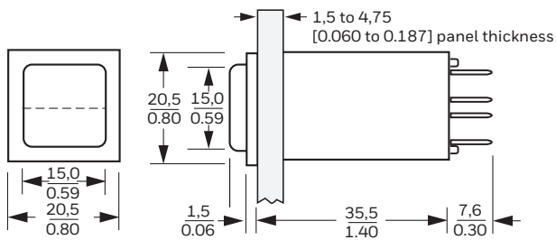
Figure 44. AML41 Series Dimensions, mm [in] or mm/in
