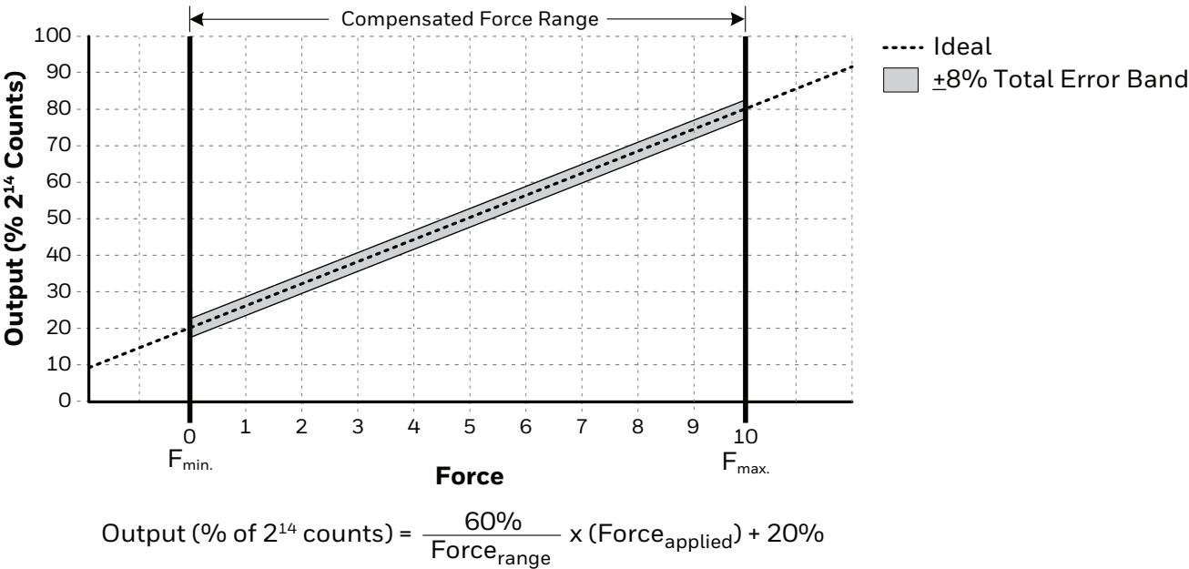
FIGURE 1. TRANSFER FUNCTION LIMITS
